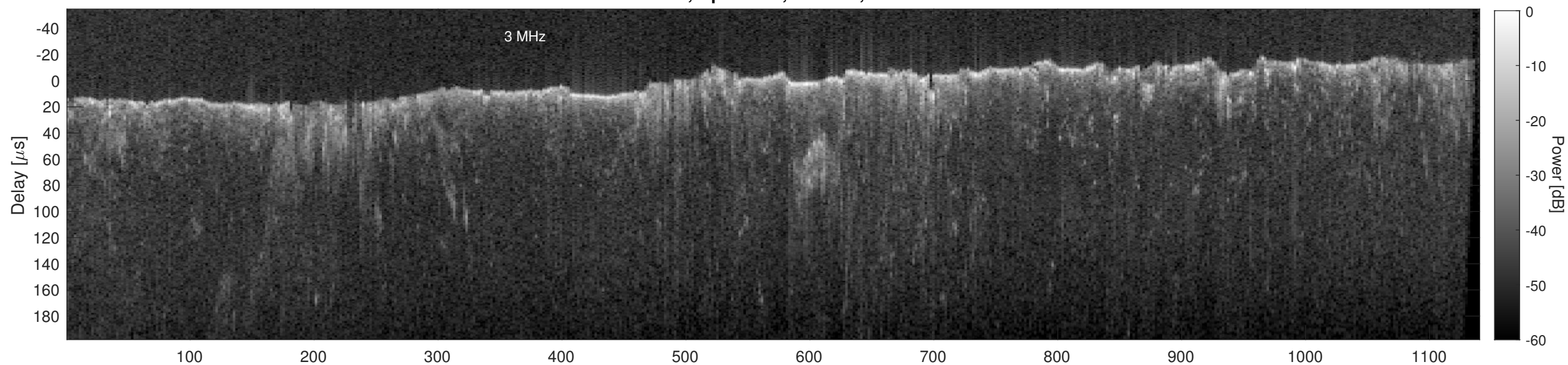
Orbit 11276, Cluttergram
