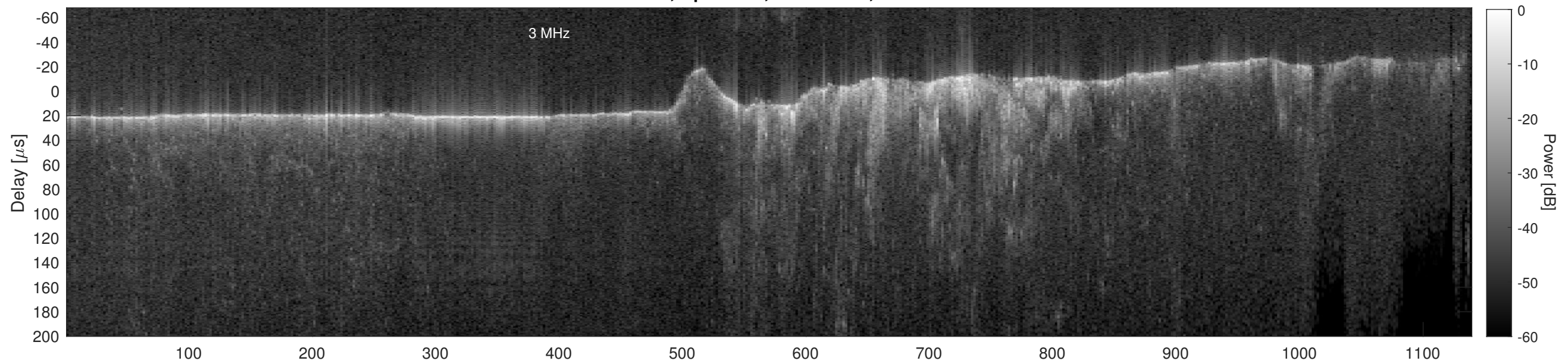
Orbit 11278, Cluttergram
