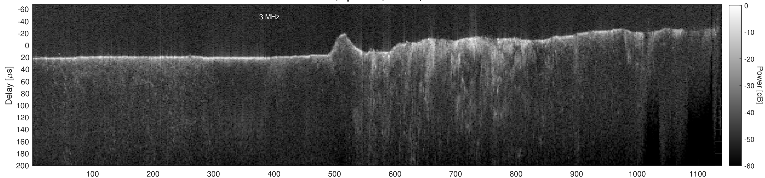
Orbit 11278, Cluttergram
