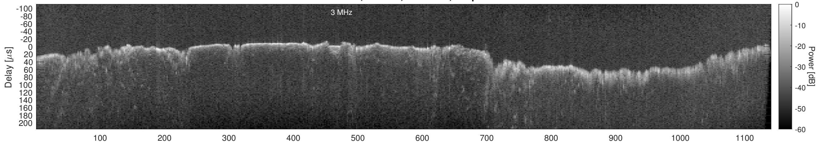
Orbit 11279, Window, Channel 2, Optimized
