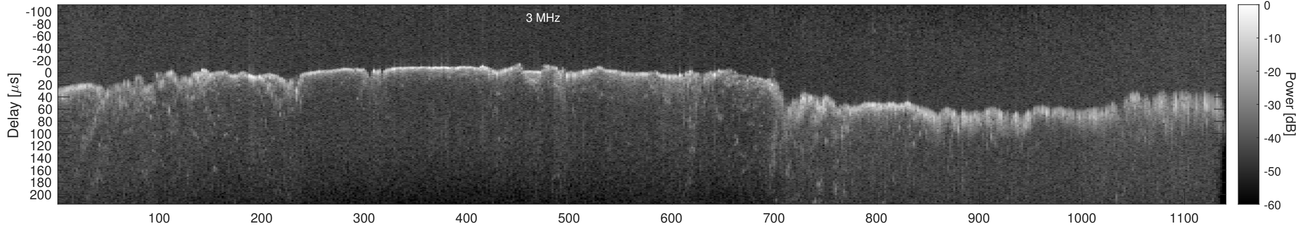
Orbit 11279, Window, Channel 2, Chapman
