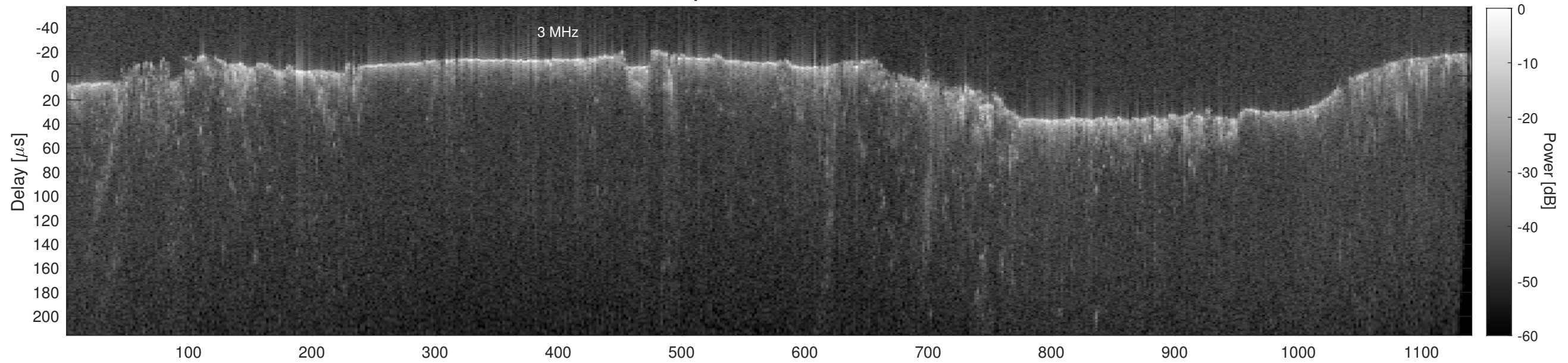
Orbit 11279, Cluttergram
