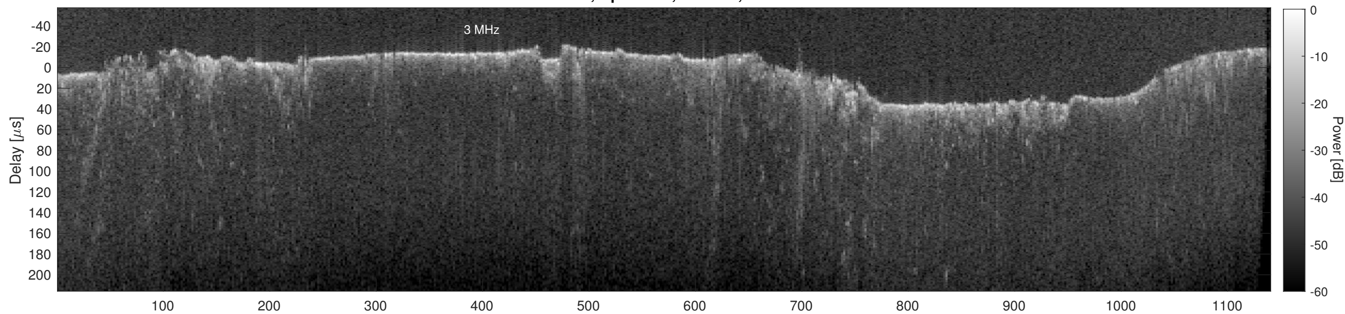
Orbit 11279, Cluttergram
