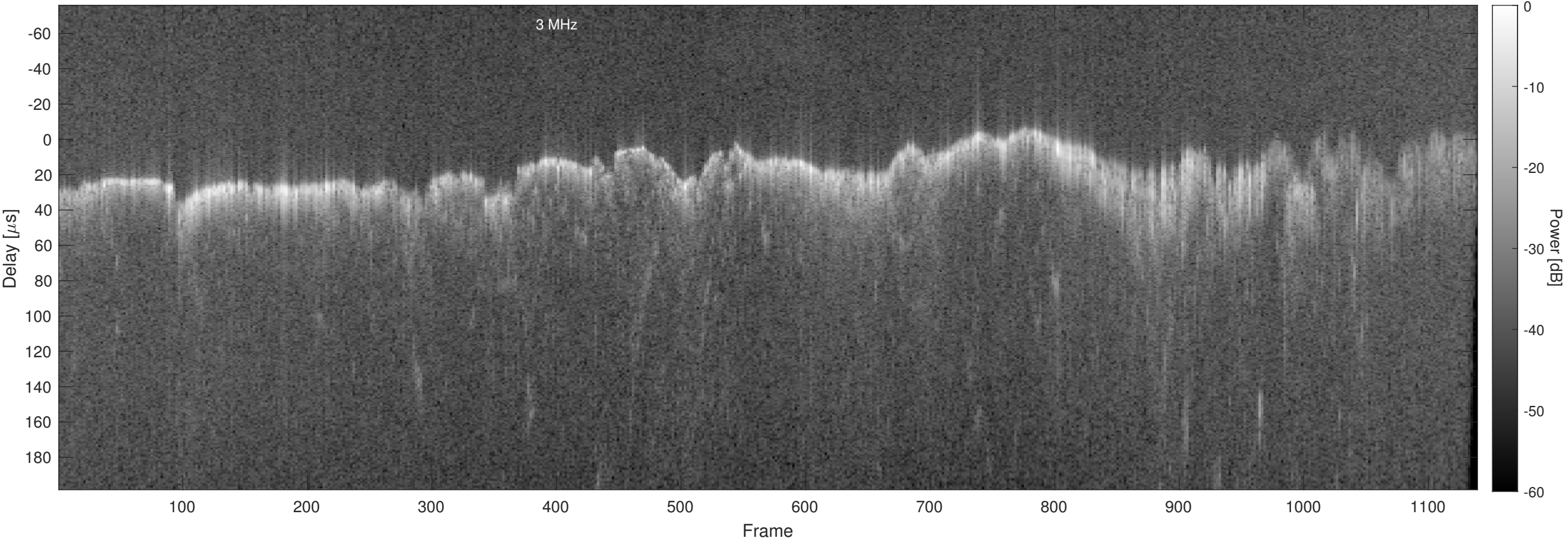
Orbit 11280, Chapman, No Window, Channel 2
