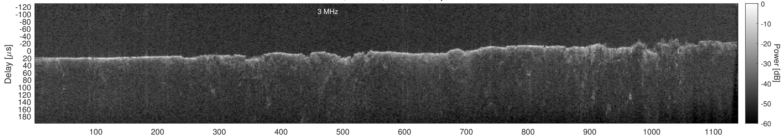
Orbit 11280, Cluttergram
