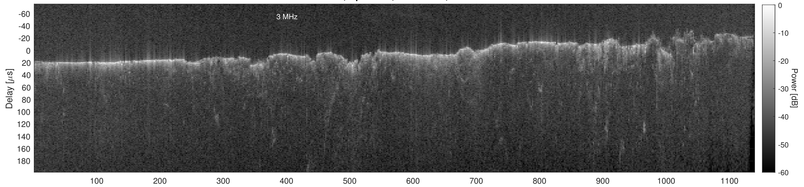
Orbit 11280, Cluttergram
