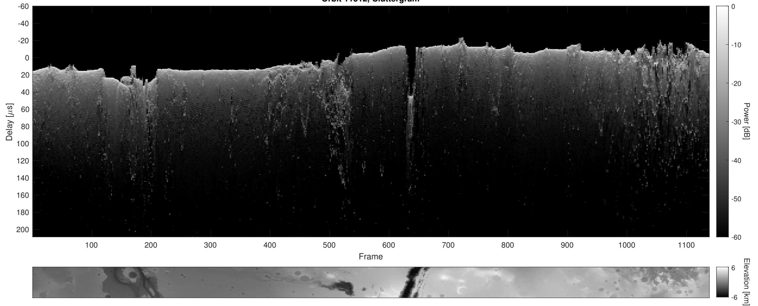
Orbit 11312, Cluttergram
