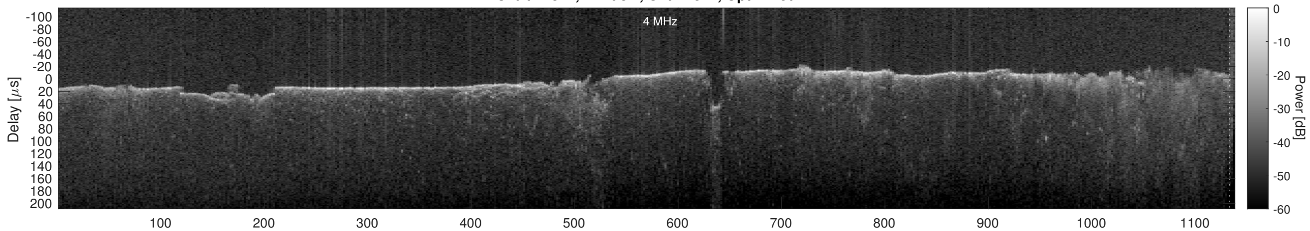
Orbit 11312, Cluttergram
