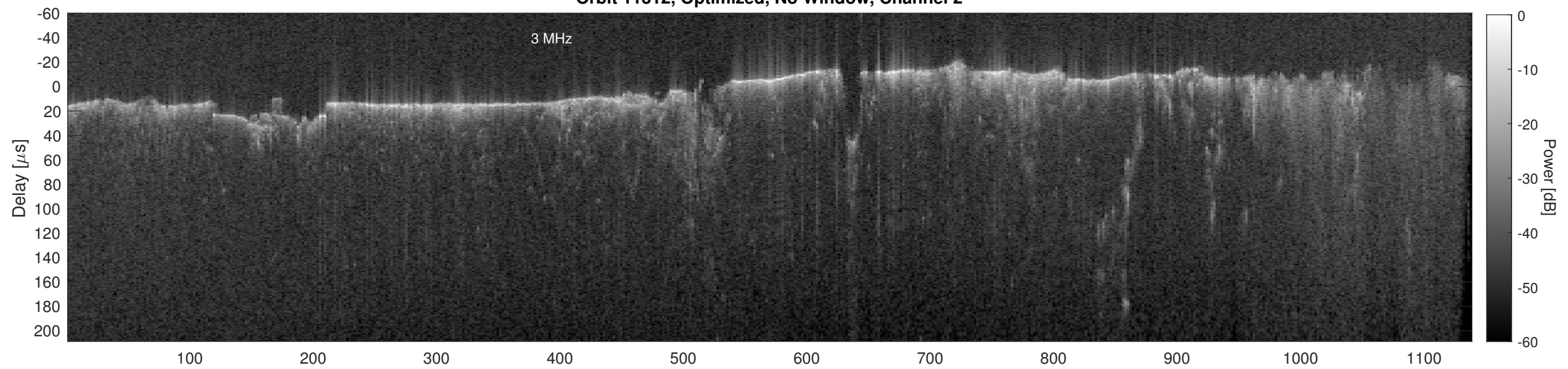
Orbit 11312, Cluttergram
