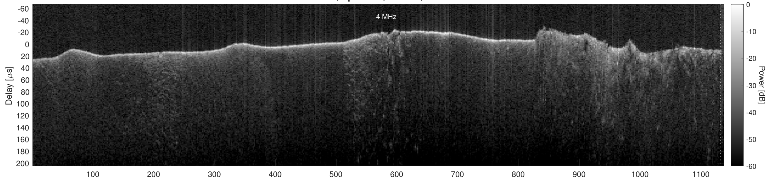
Orbit 11330, Optimized, Window, Channel 2
