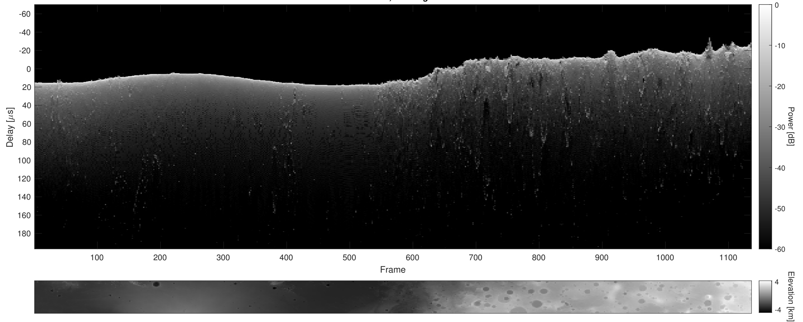
Orbit 11331, Cluttergram
