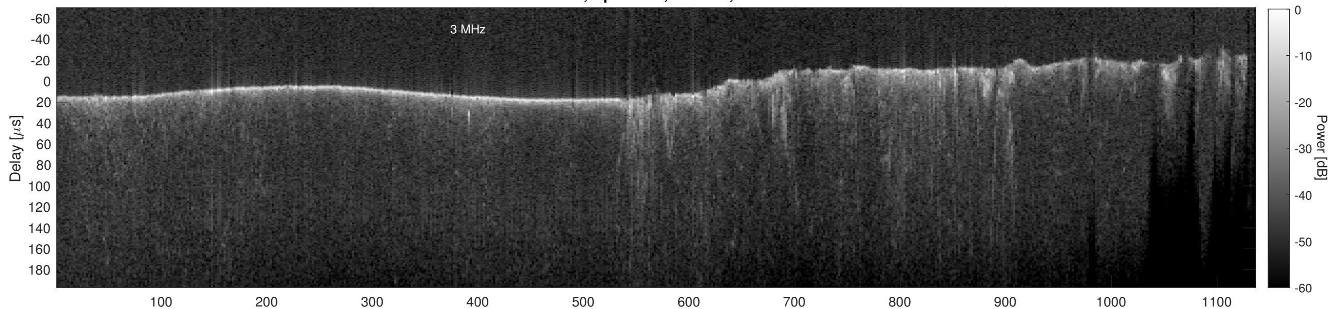
Orbit 11331, Cluttergram
