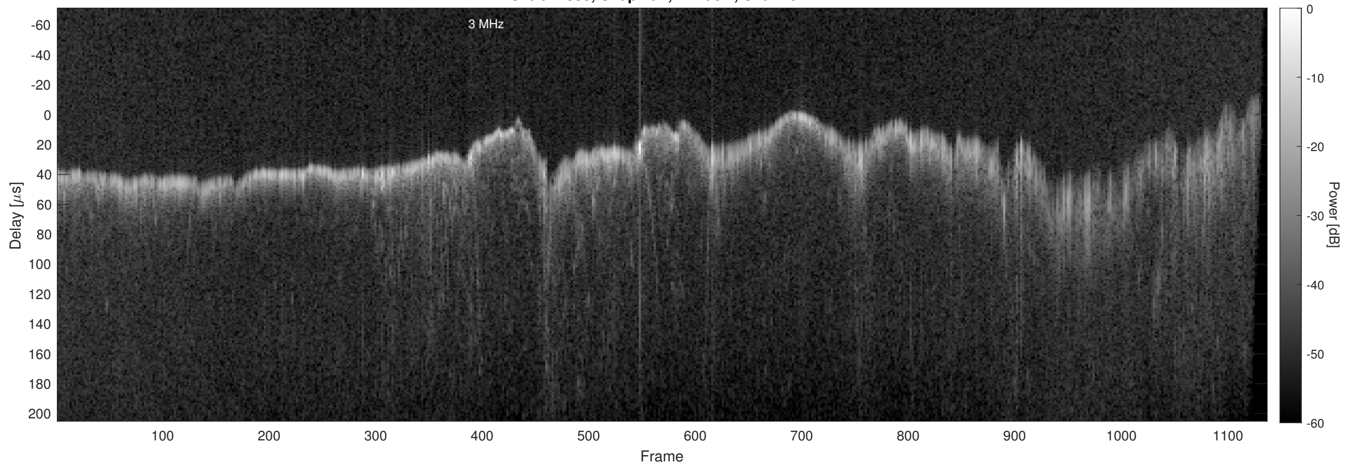
Orbit 11335, Chapman, Window, Channel 2
