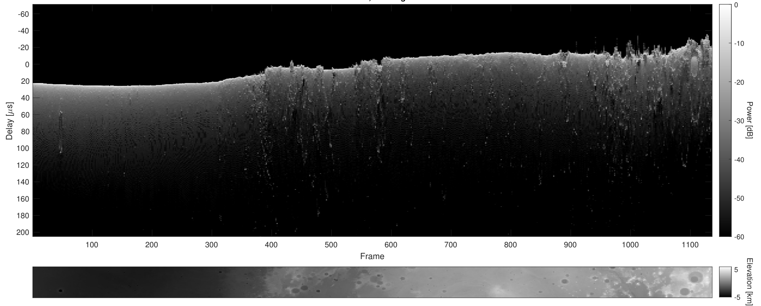
Orbit 11335, Cluttergram
