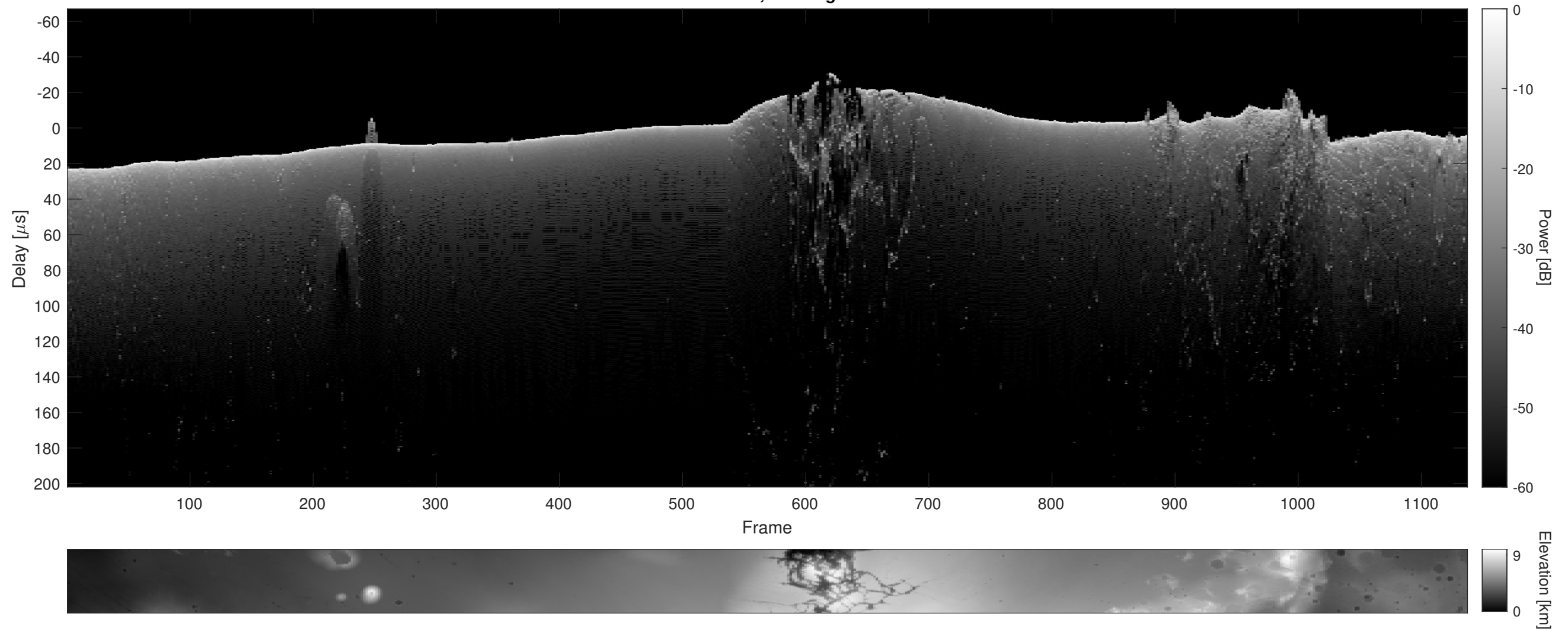
Orbit 11337, Cluttergram
