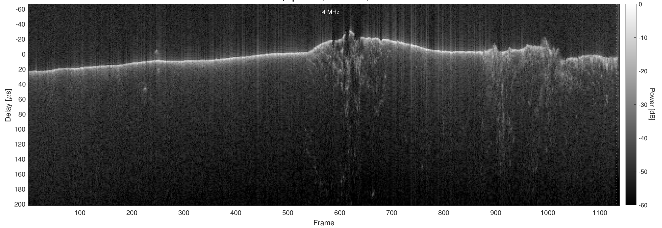
Orbit 11337, Optimized, No Window, Channel 2
