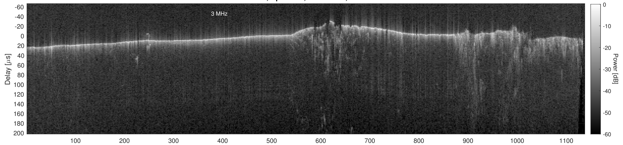
Orbit 11337, Cluttergram
