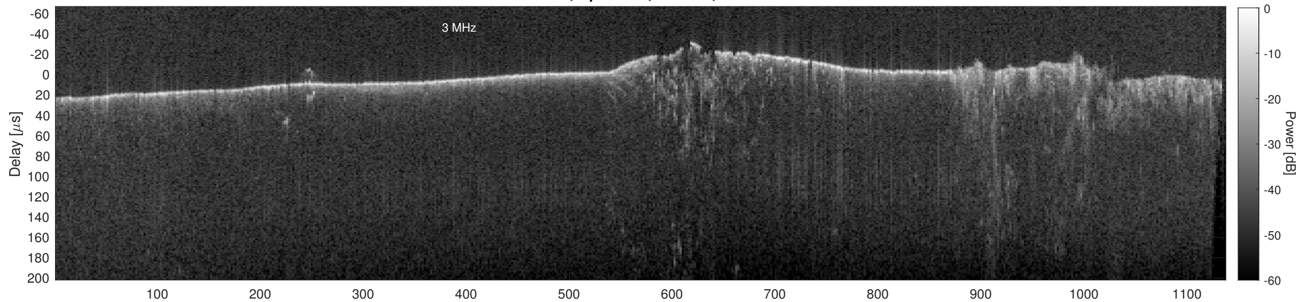
Orbit 11337, Cluttergram
