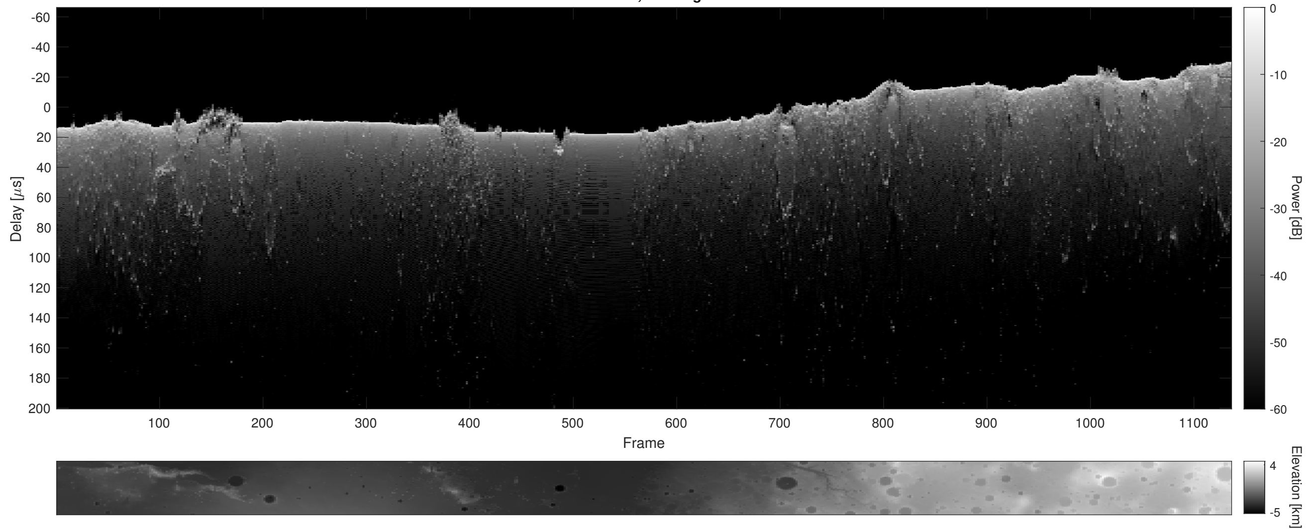
Orbit 11338, Cluttergram
