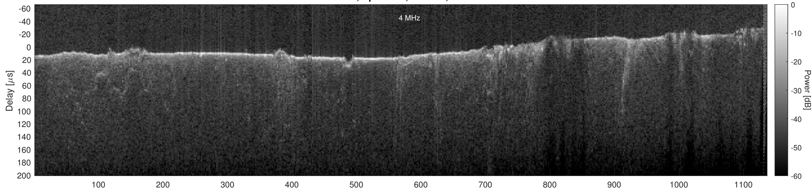
Orbit 11338, Optimized, Window, Channel 2
