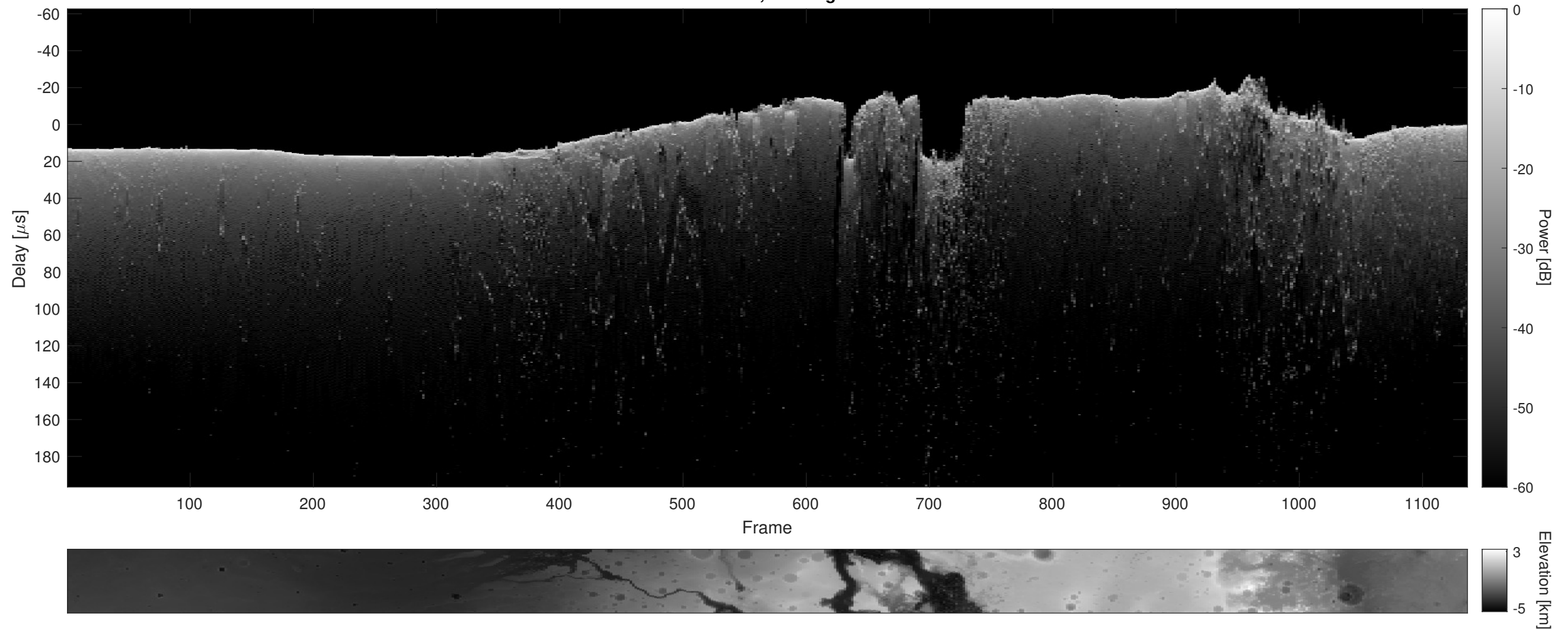
Orbit 11340, Cluttergram
