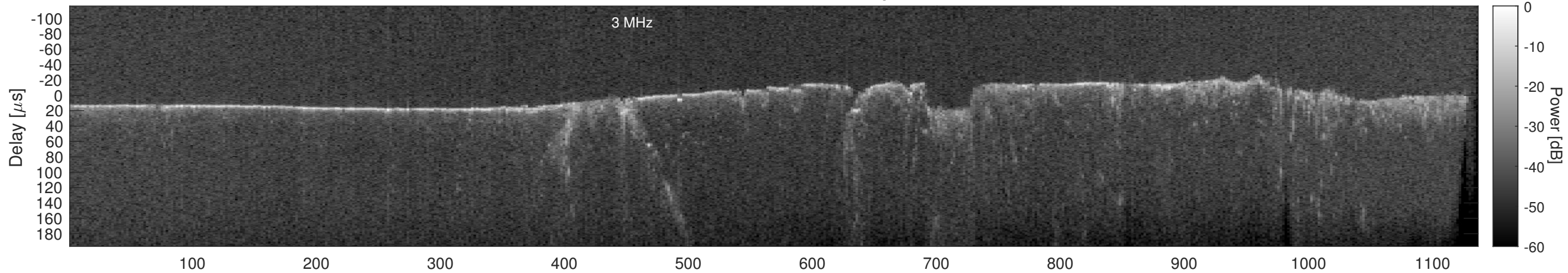
Orbit 11340, Cluttergram
