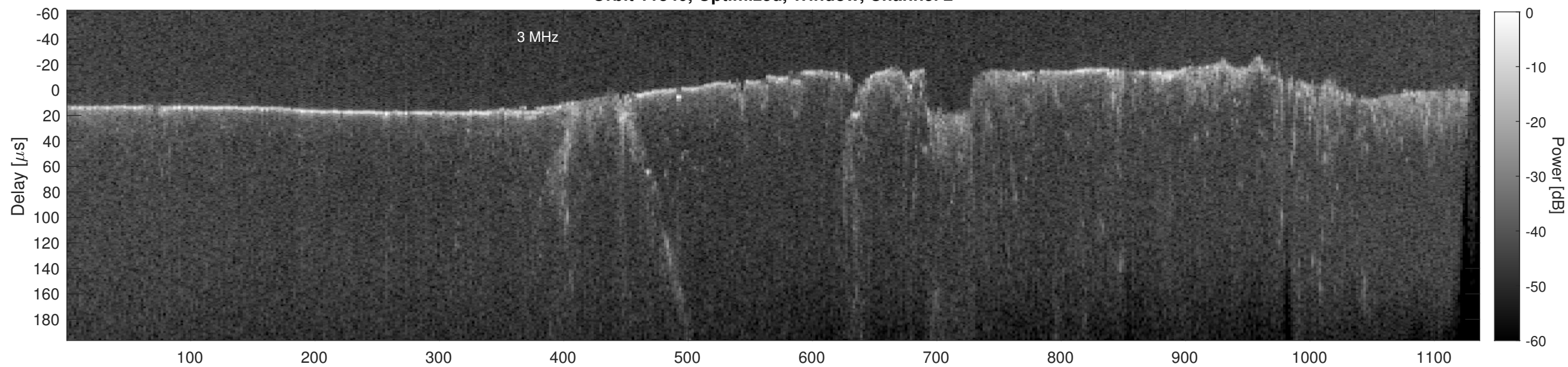
Orbit 11340, Cluttergram
