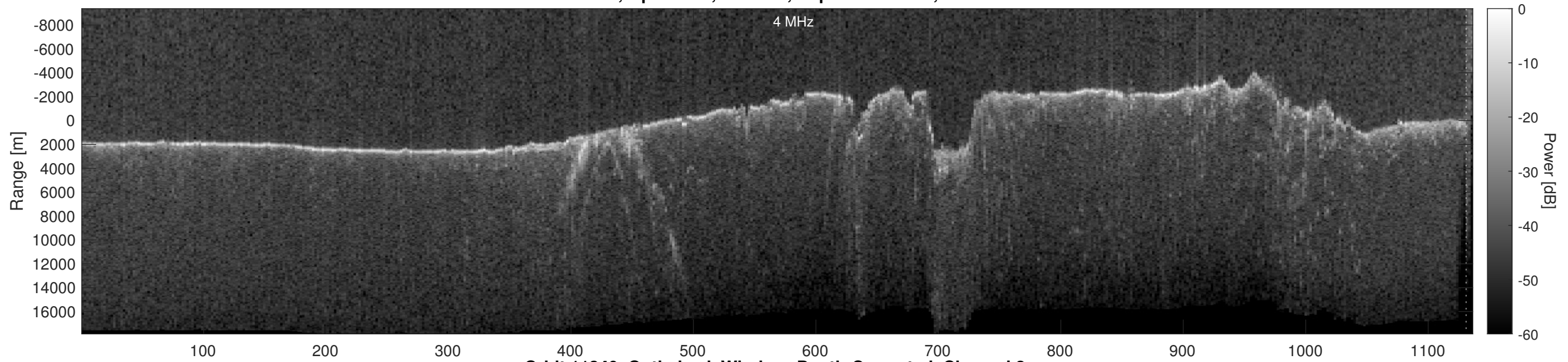
Orbit 11340, Optimized, Window, Depth-Corrected, Channel 2
