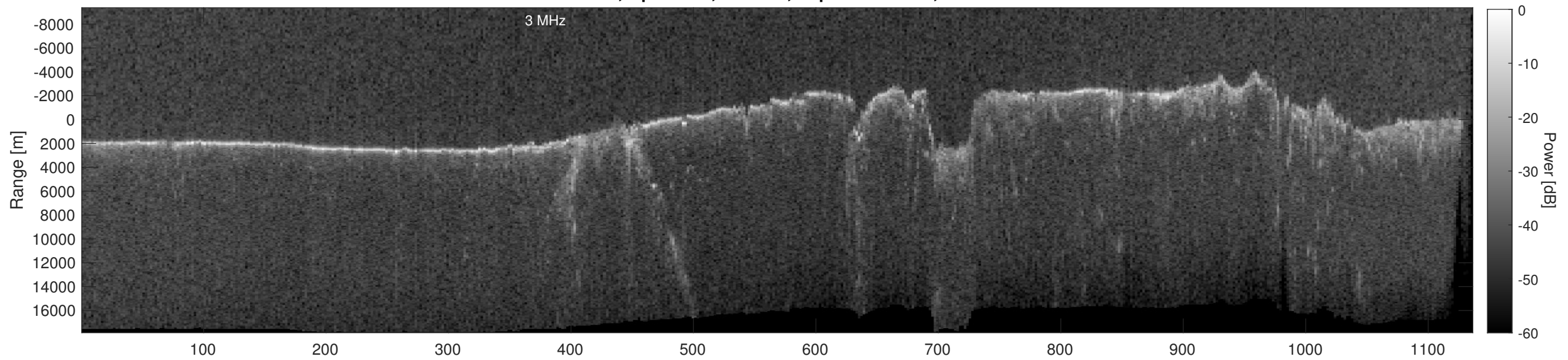
Orbit 11340, Depth-Corrected Cluttergram
