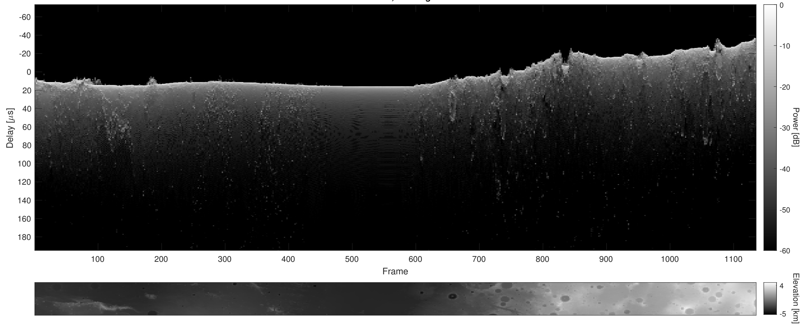
Orbit 11345, Cluttergram
