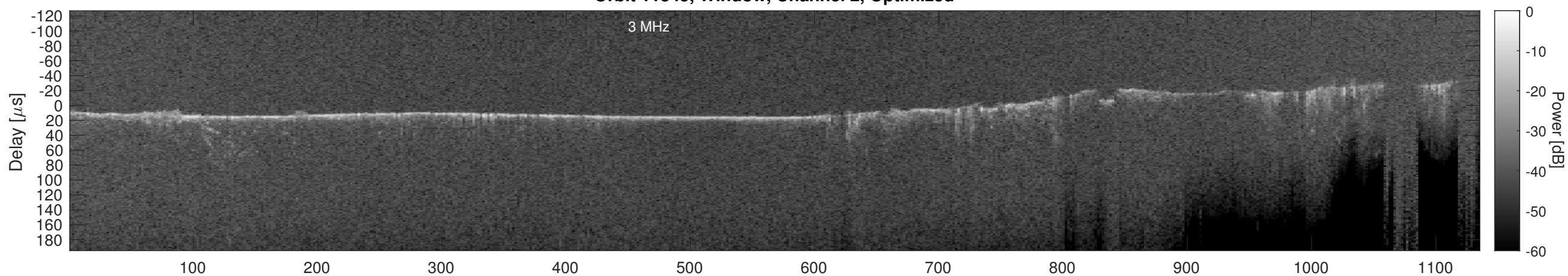
Orbit 11345, Cluttergram
