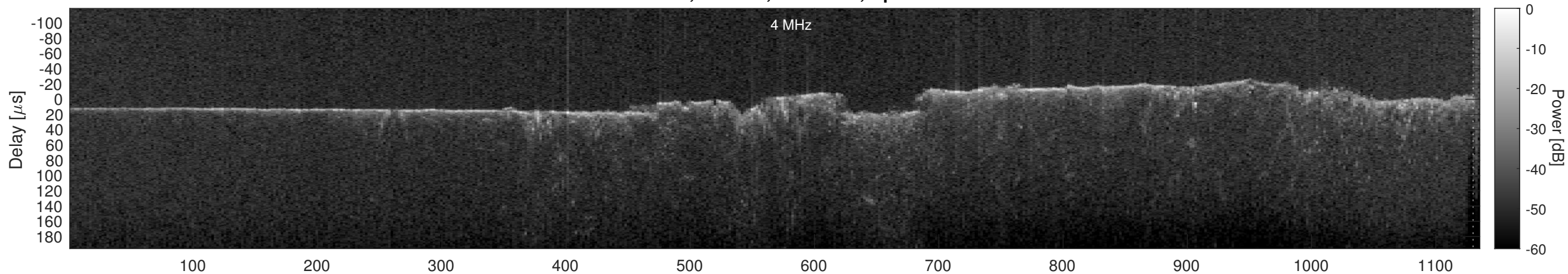
Orbit 11347, Cluttergram
