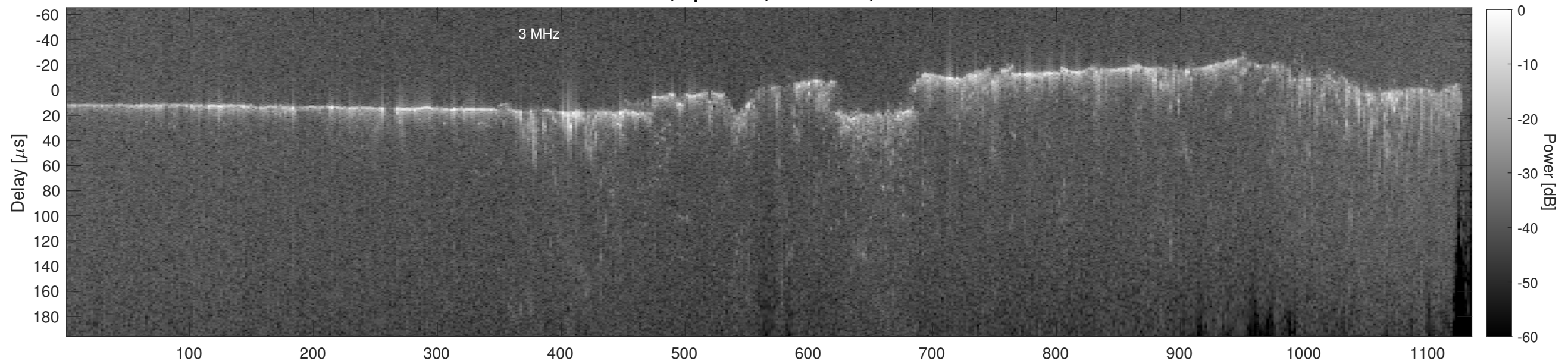
Orbit 11347, Cluttergram
