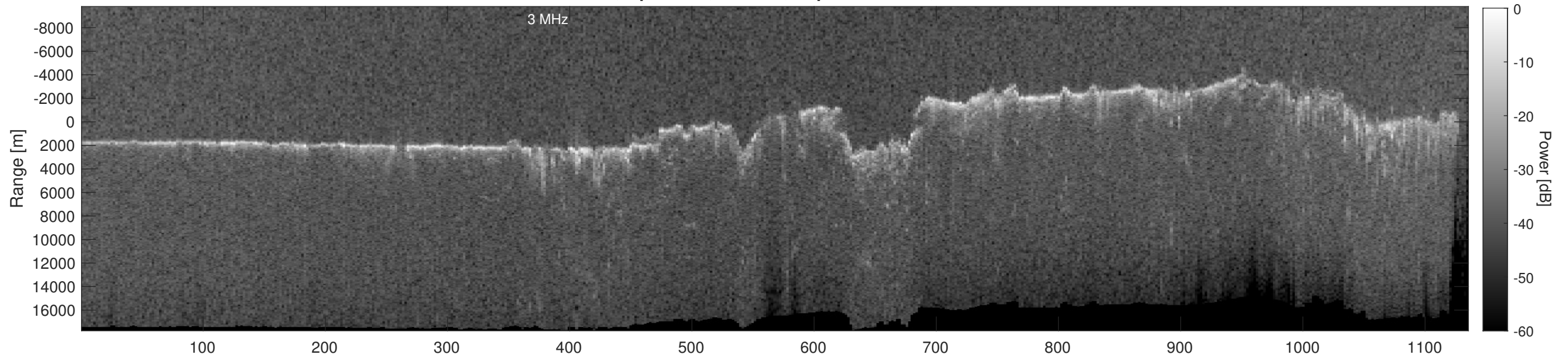
Orbit 11347, Depth-Corrected Cluttergram
