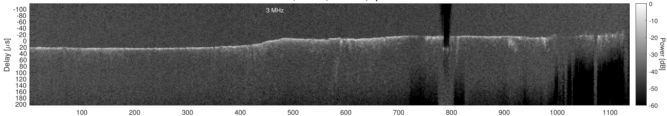
Orbit 11349, Cluttergram
