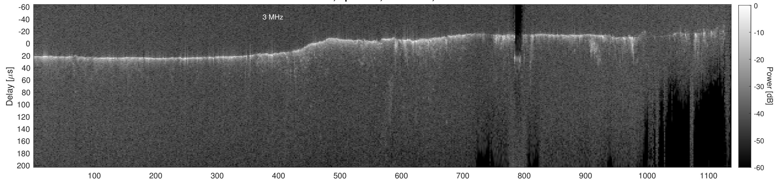
Orbit 11349, Cluttergram
