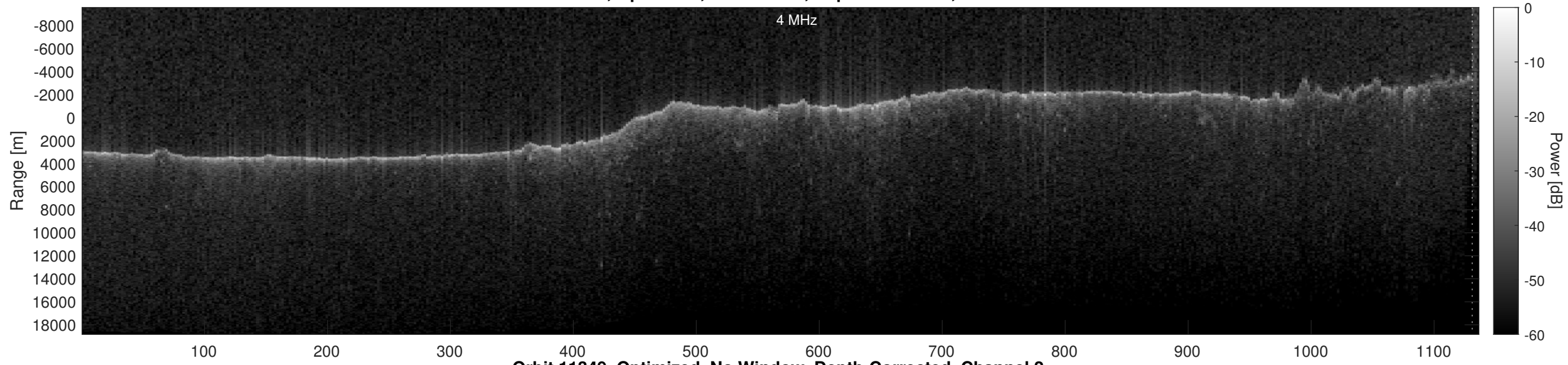
Orbit 11349, Optimized, No Window, Depth-Corrected, Channel 2
