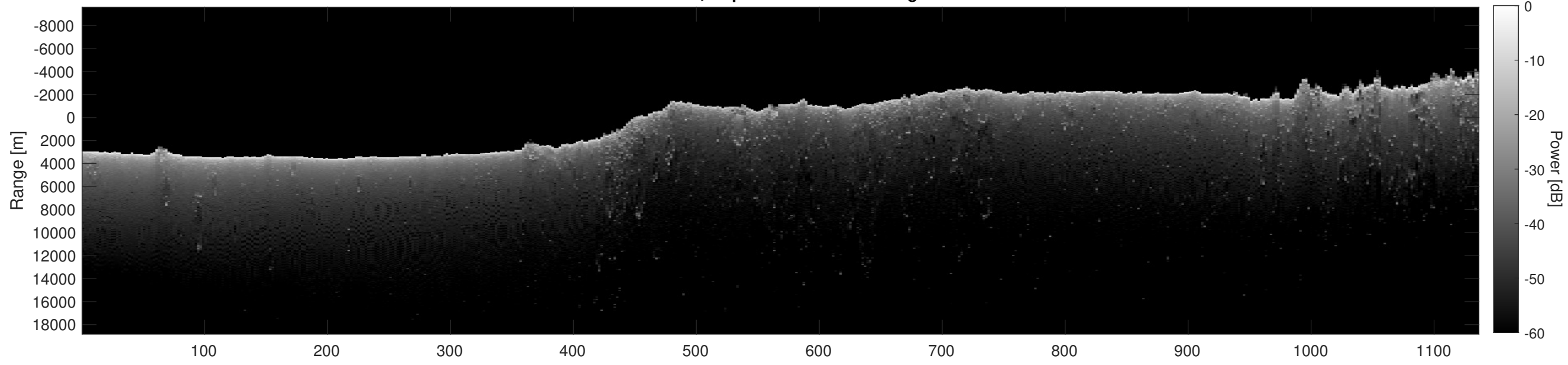
Orbit 11349, Depth-Corrected Cluttergram
