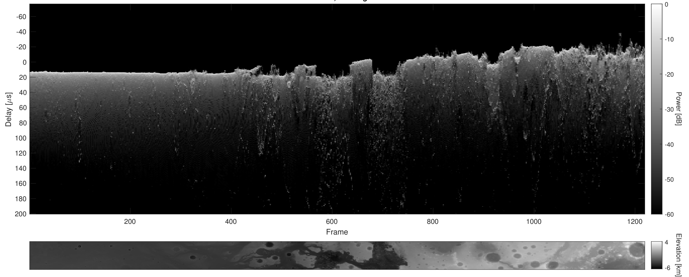
Orbit 11354, Cluttergram
