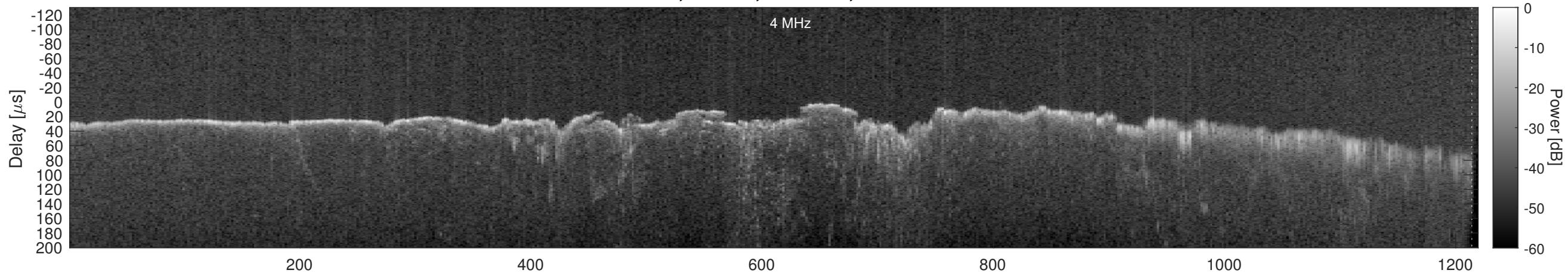
Orbit 11354, Window, Channel 2, Chapman
