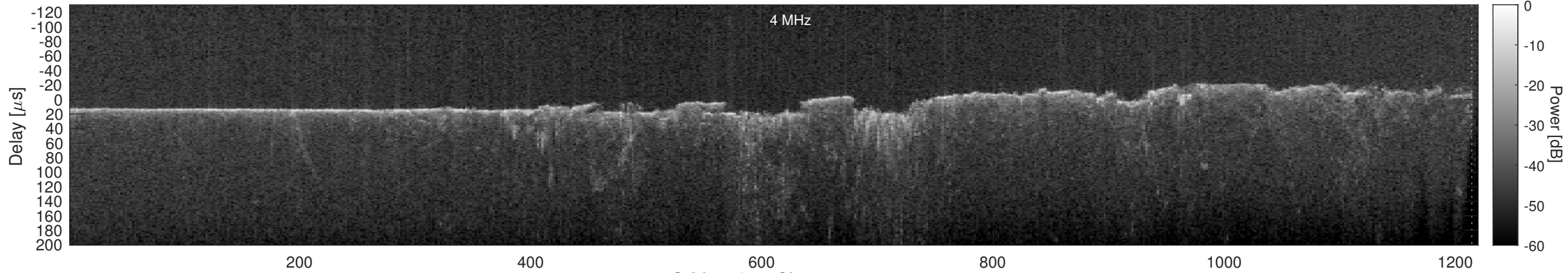
Orbit 11354, Cluttergram
