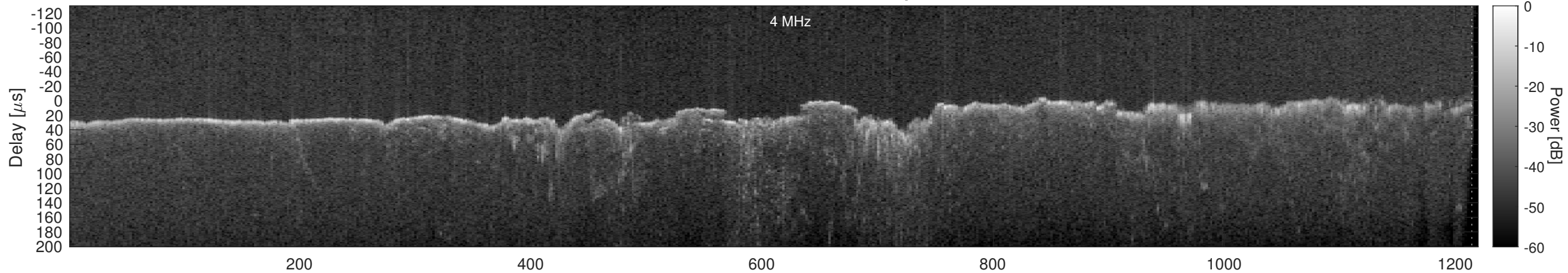
Orbit 11354, Window, Channel 2, Optimized
