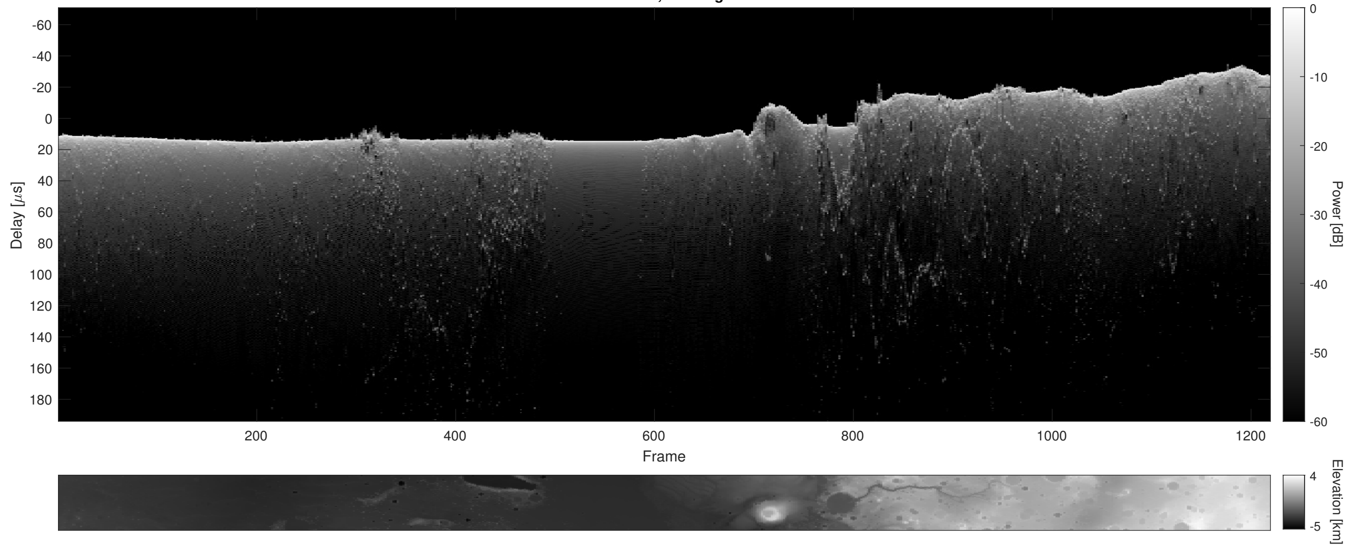
Orbit 11359, Cluttergram
