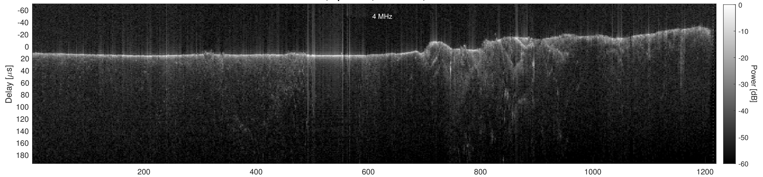
Orbit 11359, Cluttergram
