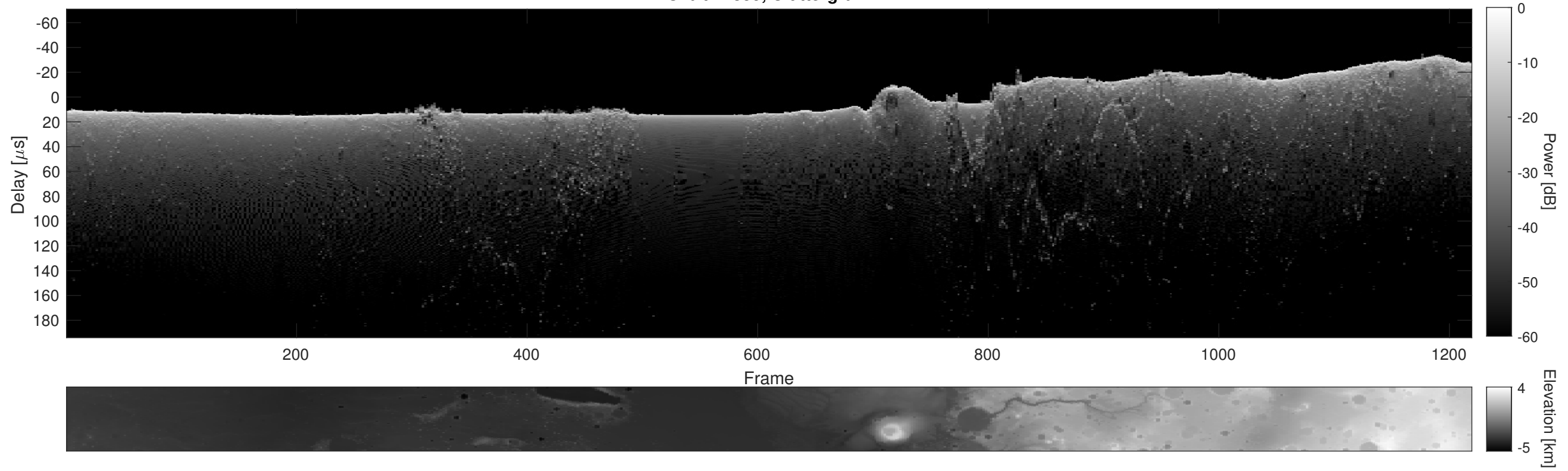
Orbit 11359, Cluttergram
