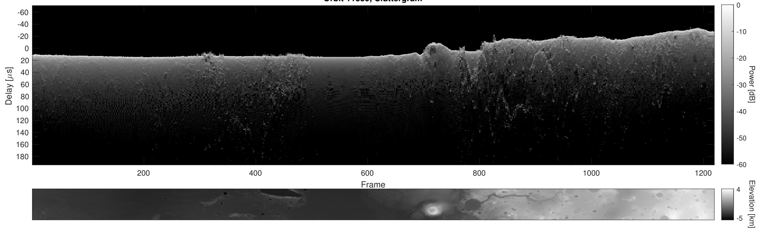
Orbit 11359, Cluttergram
