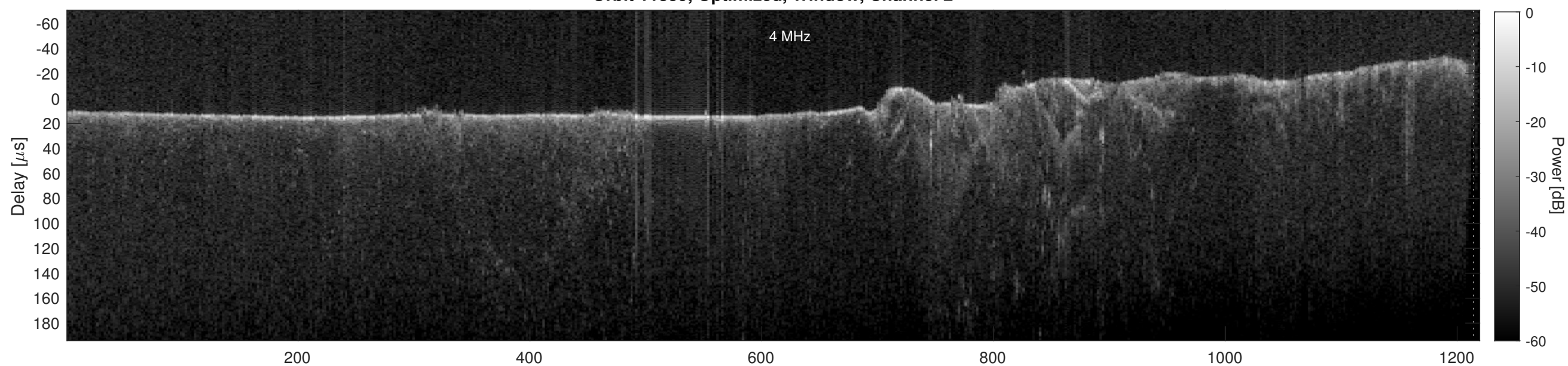
Orbit 11359, Cluttergram
