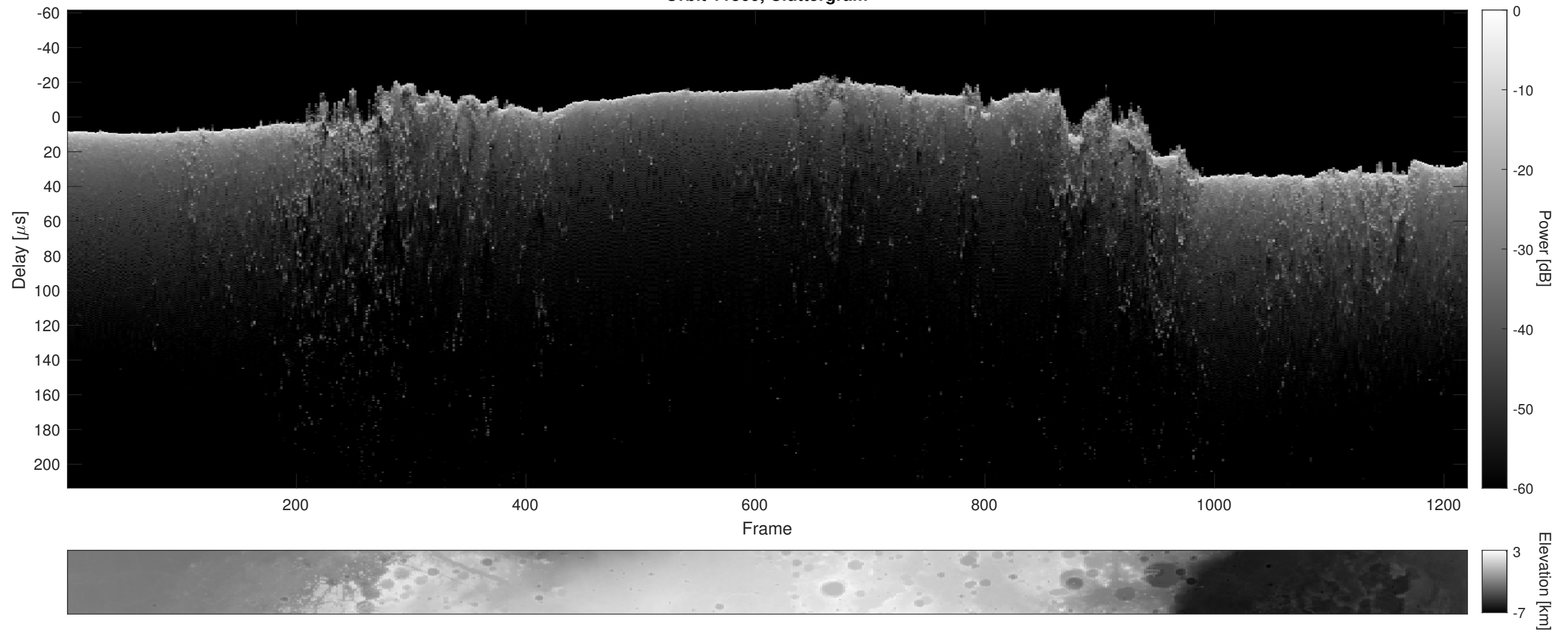
Orbit 11360, Cluttergram
