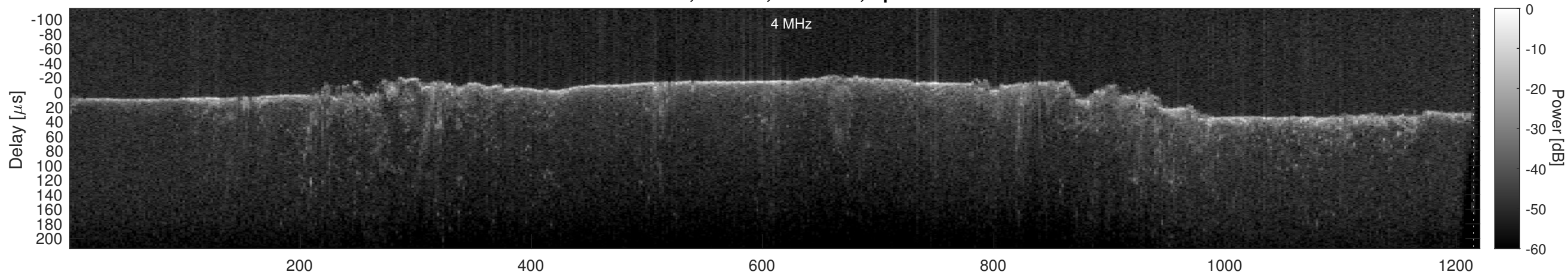
Orbit 11360, Cluttergram
