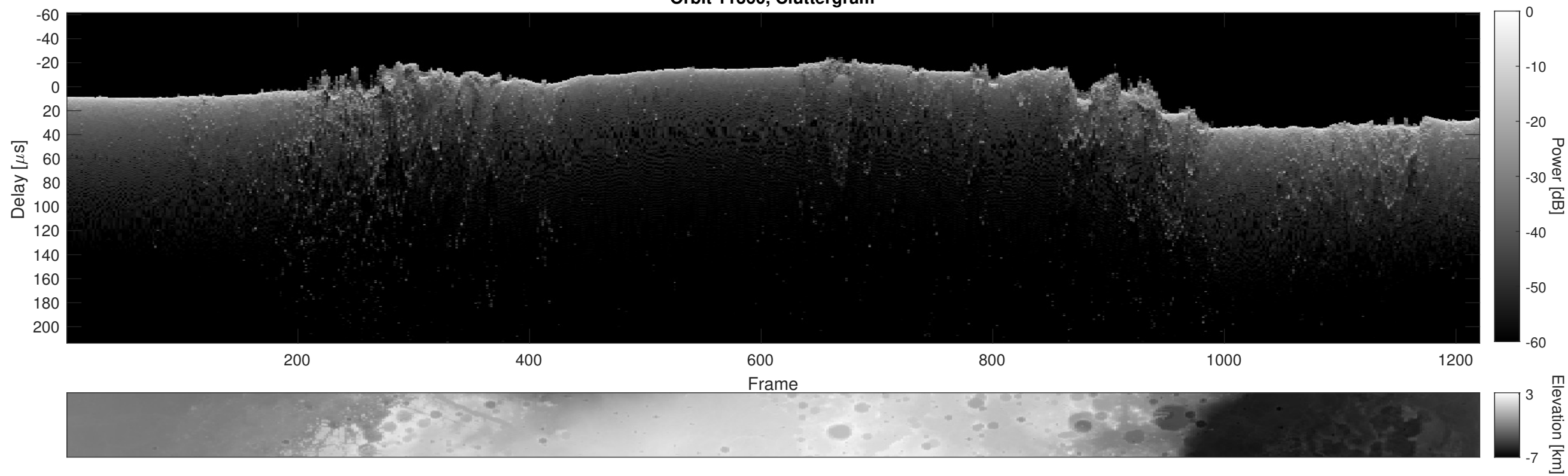
Orbit 11360, Cluttergram
