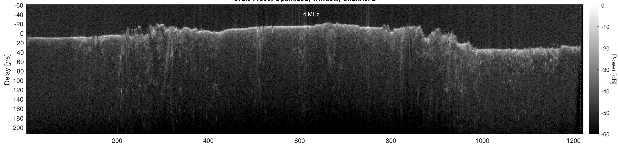
Orbit 11360, Cluttergram
