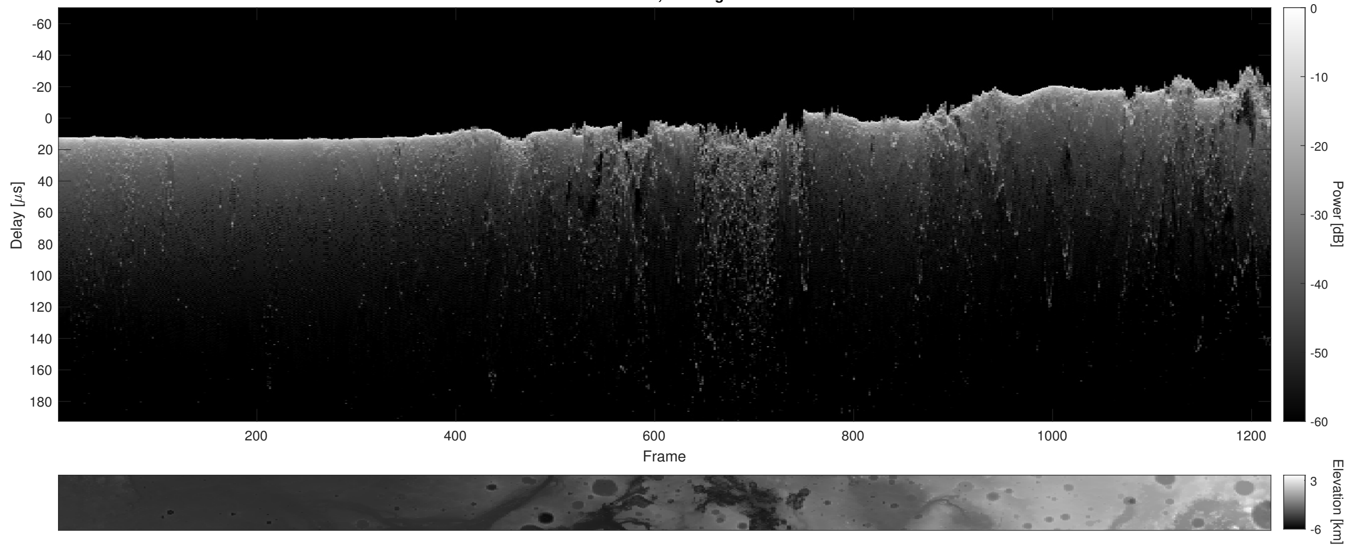
Orbit 11361, Cluttergram
