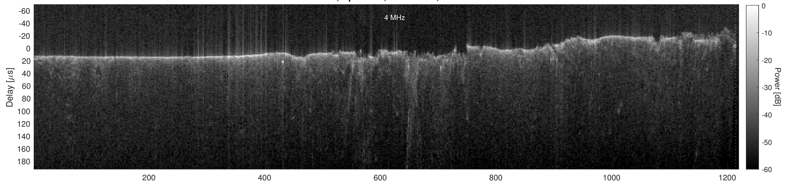
Orbit 11361, Cluttergram
