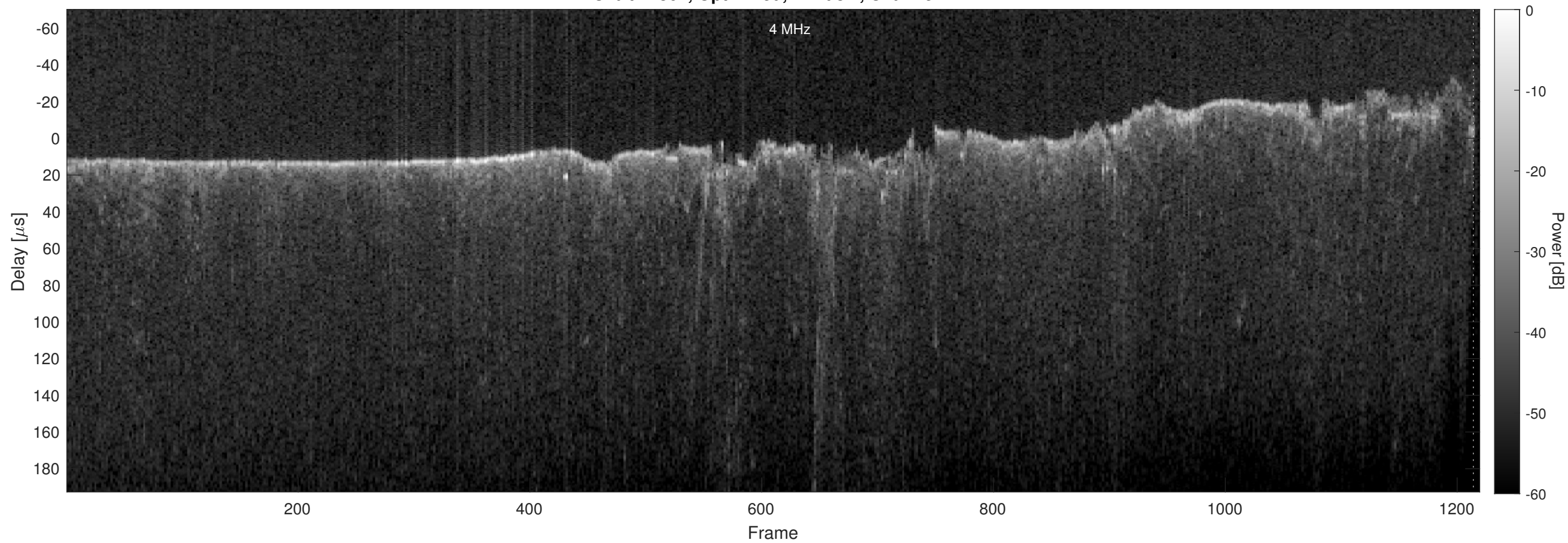
Orbit 11361, Optimized, Window, Channel 2
