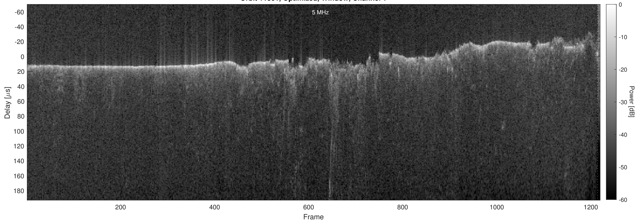
Orbit 11361, Optimized, Window, Channel 2
