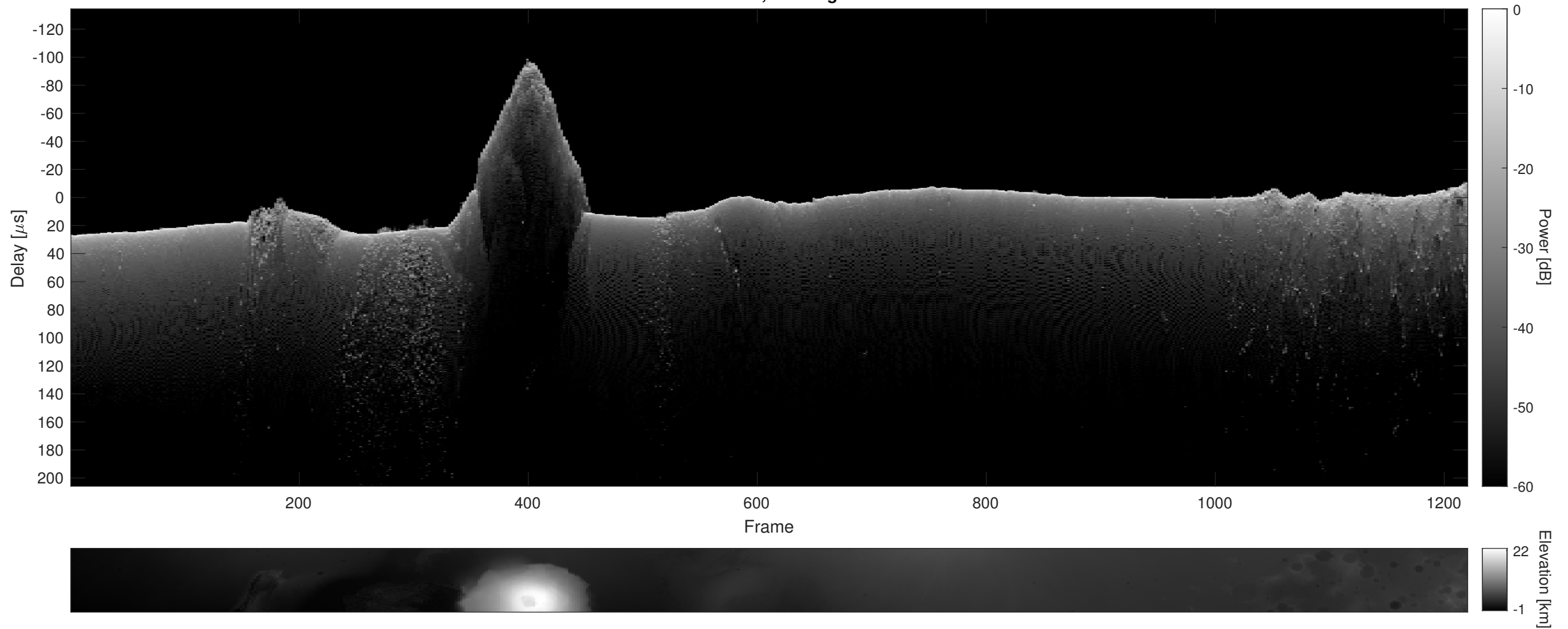
Orbit 11362, Cluttergram
