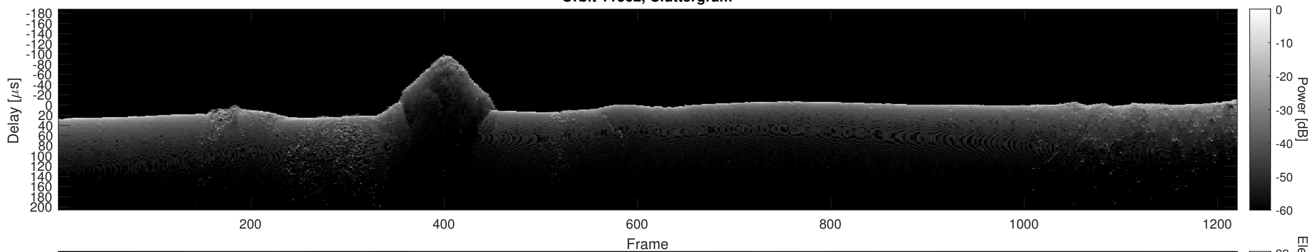
Orbit 11362, Cluttergram
