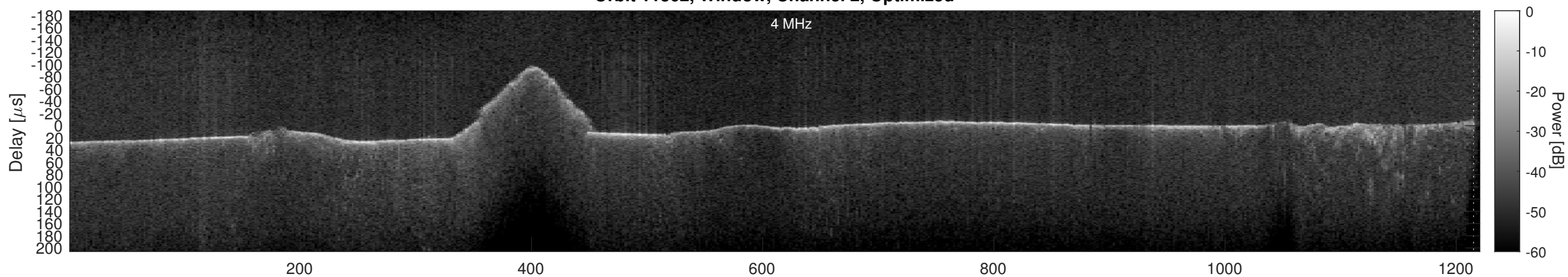
Orbit 11362, Cluttergram
