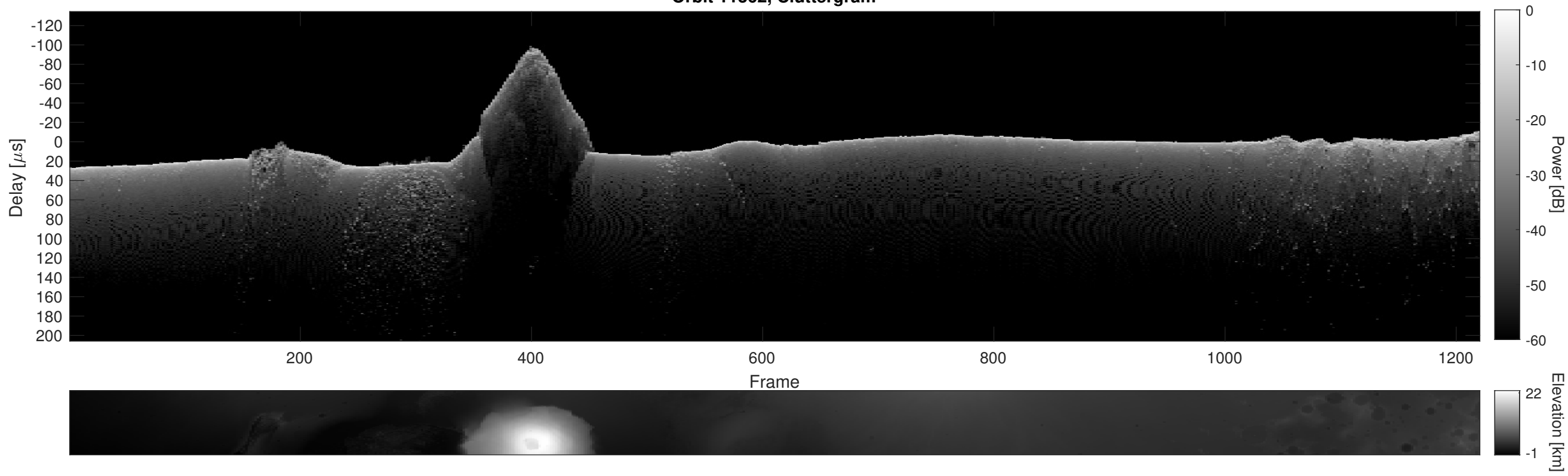
Orbit 11362, Cluttergram
