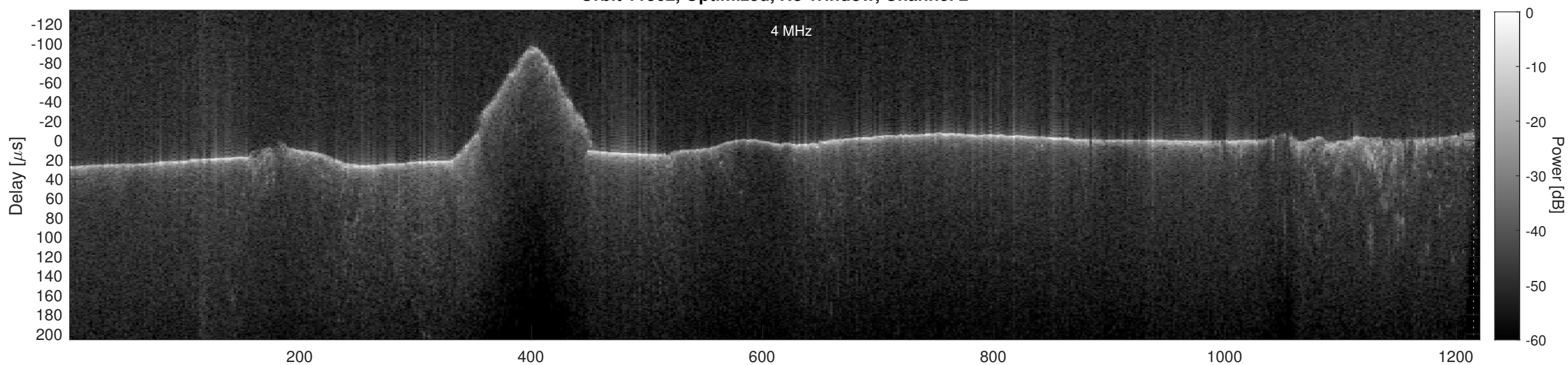
Orbit 11362, Cluttergram
