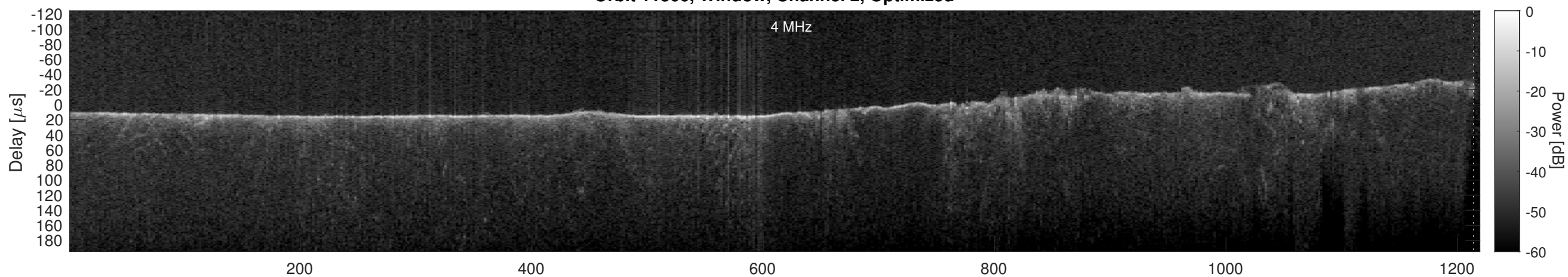
Orbit 11366, Cluttergram
